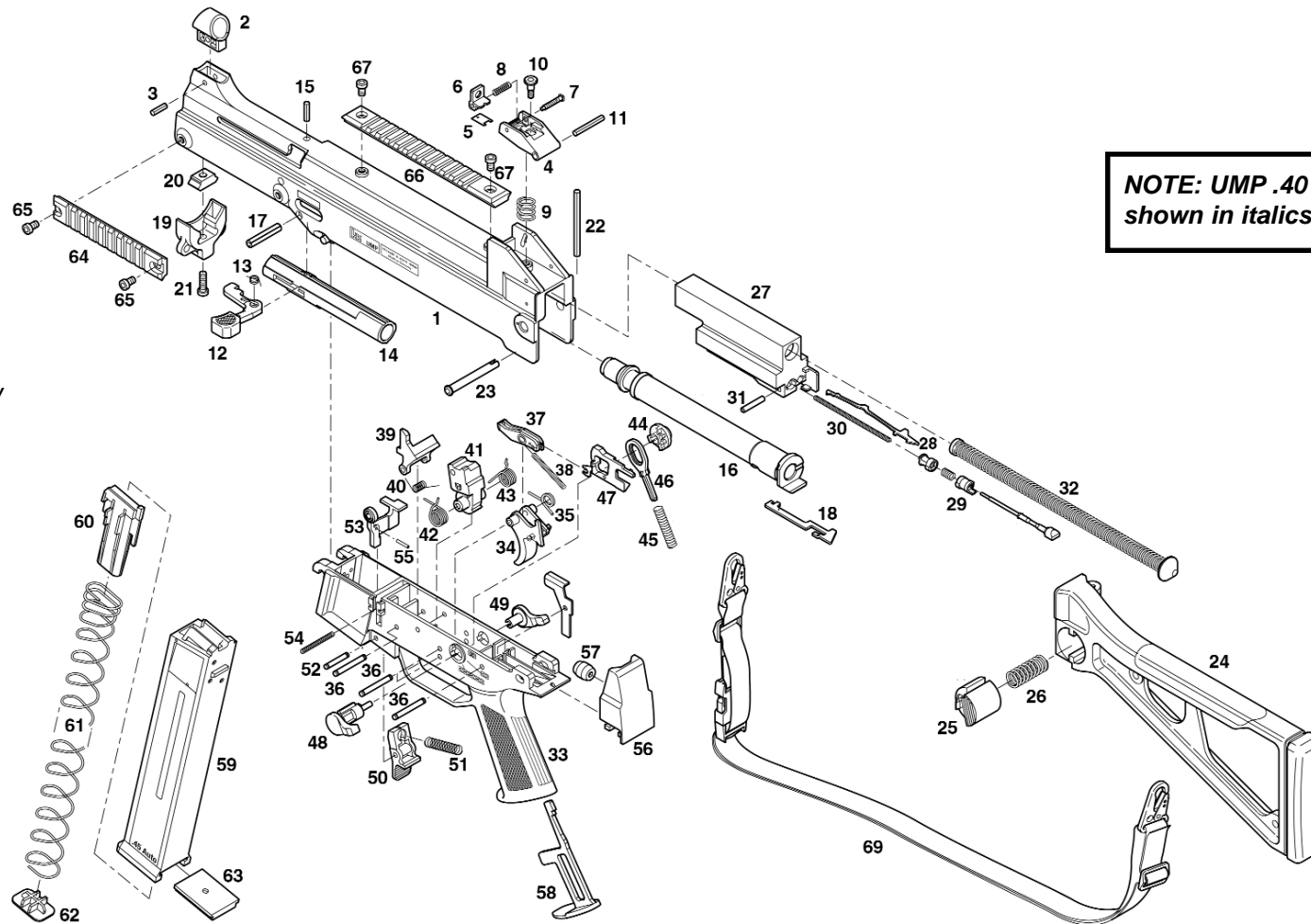
Fig. 43 UMP .45 ACP & .40 S&W
