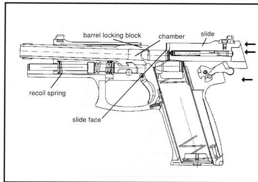
Figure 8 Feeding
