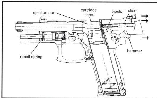
Figure 7 Ejection
