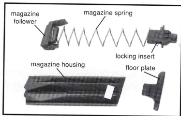
Figure 11B 10-Round Civilian Magazine (Disassembled)
