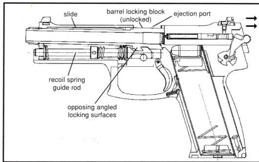
Figure 6 Unlocking
