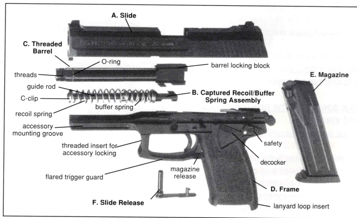
Figure 3 Major Assembly Groups
