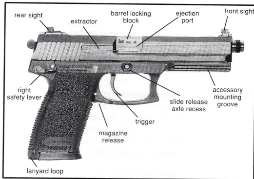
Figure 2 Right View
