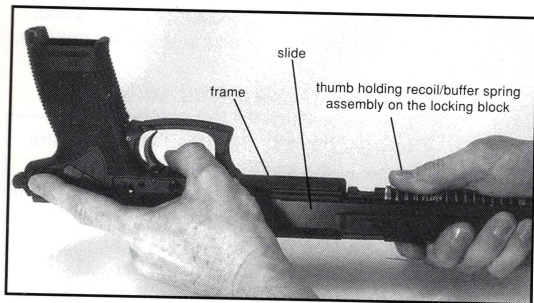
Figure 13 Correct Position for Holding Slide for Reassembly
