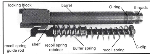
Figure 12 Proper Position for the Captured Recoil/Buffer Spring Assembly on the Barrel Locking Block
