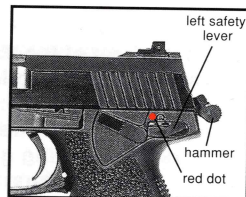
Figure 4a "Safe" Position Figure 4b "Fire" Position The safety lever cannot be placed in the "safe" (up) position if the hammer is uncocked (down).
