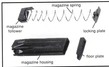
Figure 11A Assembly of Magazine Follower & Spring (12-Round Law Enforcement Magazine)
