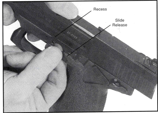
Figure 10 Removing or Installing the Slide Release
