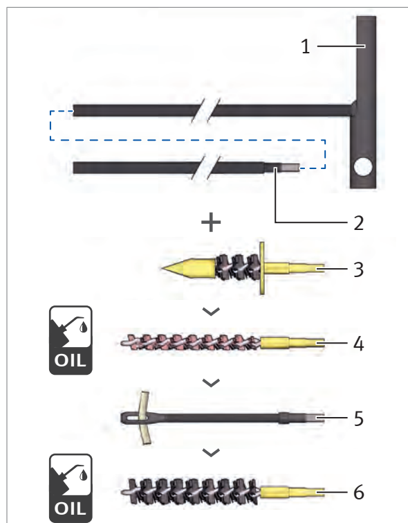
Fig. 30: Clean barrel
