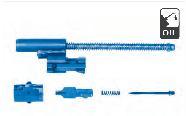
Fig. 31: Lubrication points of bolt group
