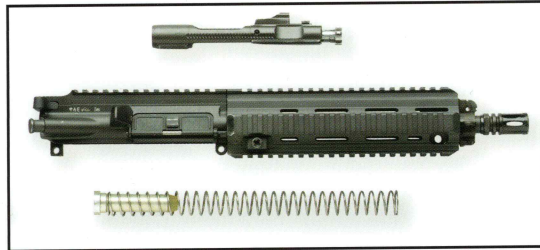
Drop-on HK416 upper receiver kits are available to retrofit existing M16 and M4-type weapons in the field in seconds without tools.
